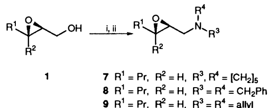
Scheme 2 Reagents and conditions: i, TsCl, pyridine; ii, R 3 R 4 NH (2 equiv.), KI, DMF, room temp., 73–83%
